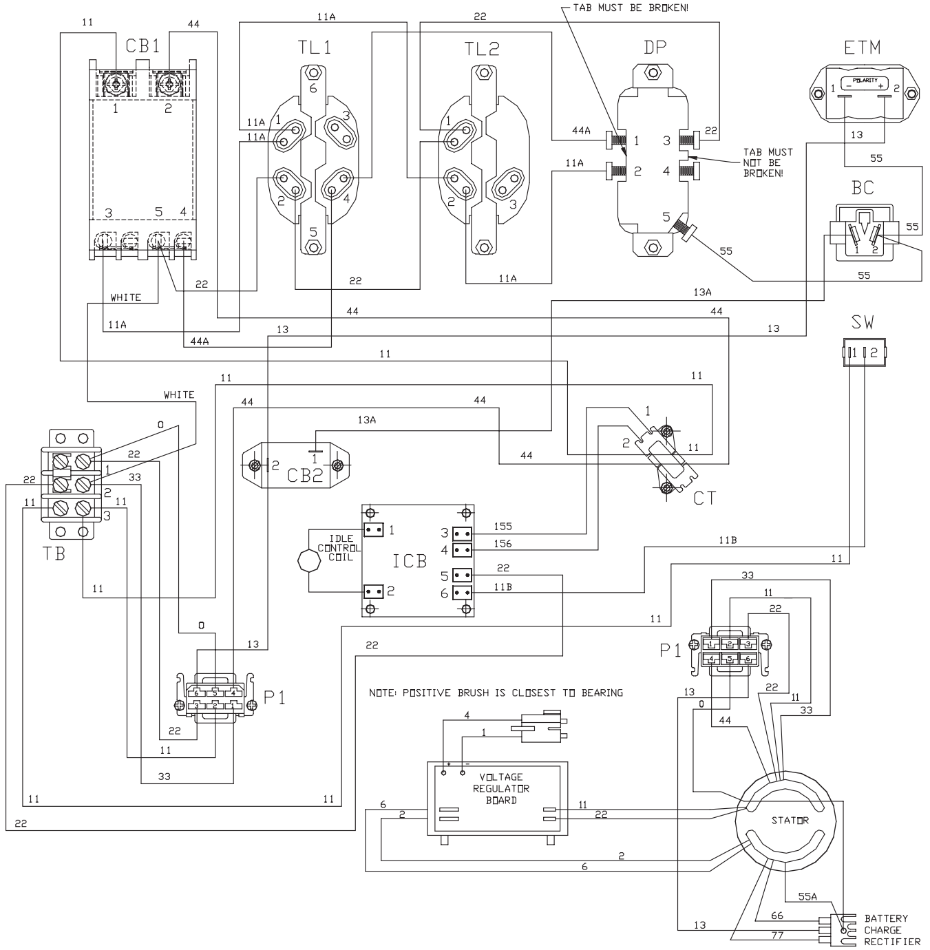
WIRE DIAGRAM
